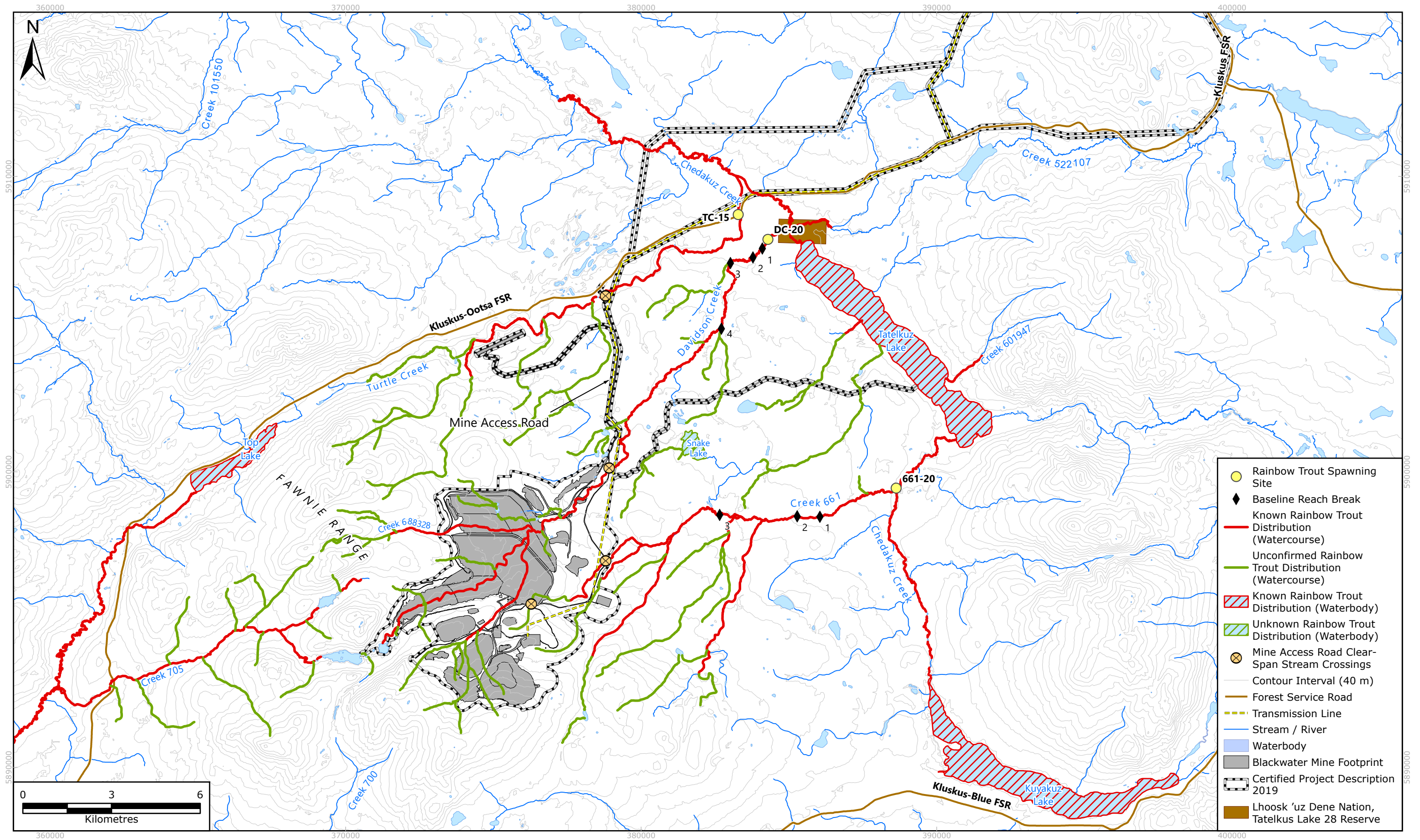
FIGURE 4.7-2 POTENTIAL RAINBOW TROUT SPAWNING LOCATIONS AND PLANNED SURVEY SITES
